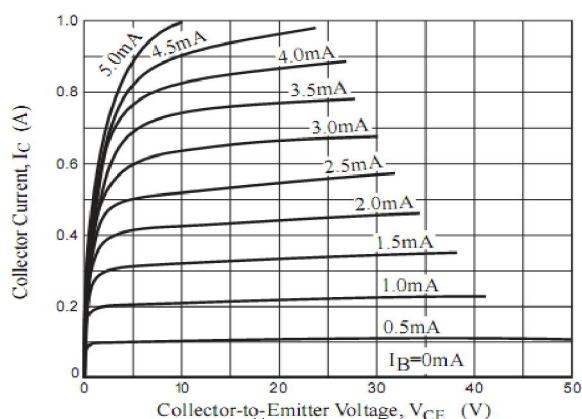
Figure 1. Static Characteristic
