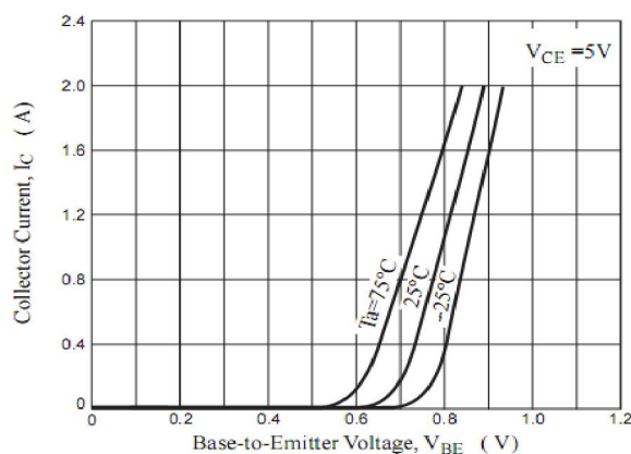
Figure 4. Base-Emitter Characteristics
