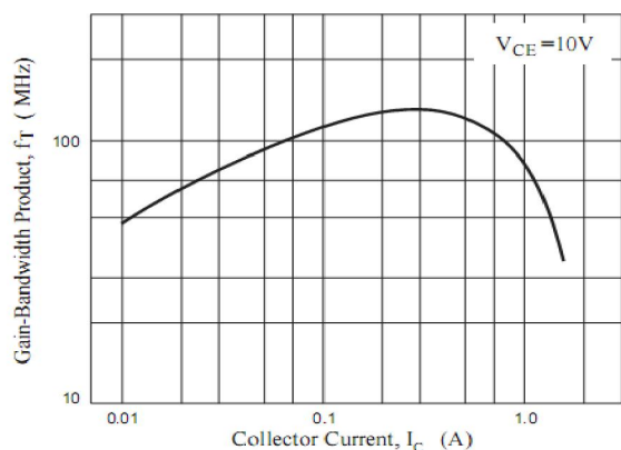
Figure 5. Current Gain Bandwidth Product
